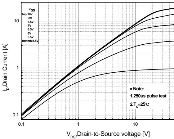
Fig 1. On-State Characteristics
