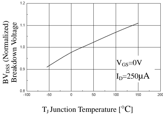
Fig 7. Breakdown Voltage Variation vs. Junction Temperature
