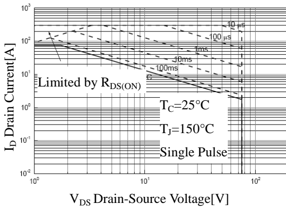
Fig 9. Maximum Safe Operating
