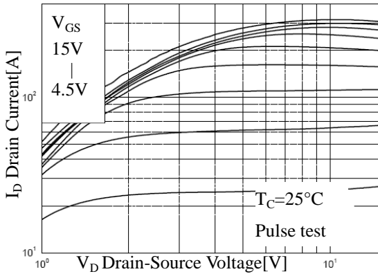
Fig 1. On-State Characteristics
