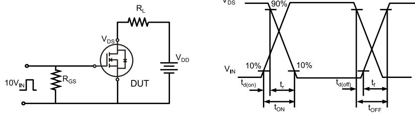
Fig. 17. Switching time test circuit & waveform
