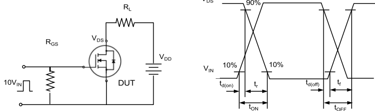
Fig. 16. Switching time test circuit & waveform
