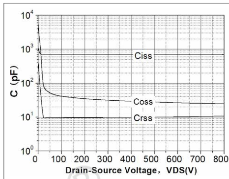
Fig. 8. Capacitance Characteristics
