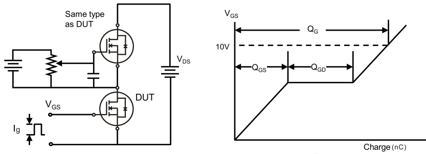
Fig. 12. Gate charge test circuit & waveform
