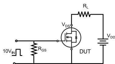
Fig. 17. Switching time test circuit & waveform
