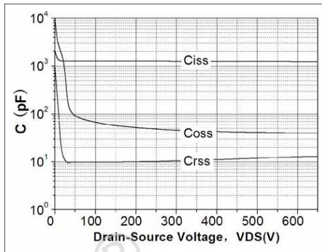
Fig. 8. Capacitance Characteristics
