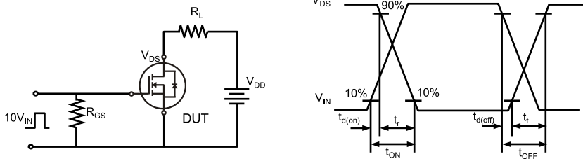
Fig. 11. Switching time test circuit & waveform
