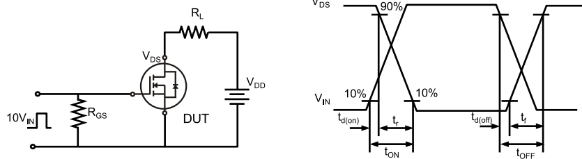
Fig. 15. Switching time test circuit & waveform
