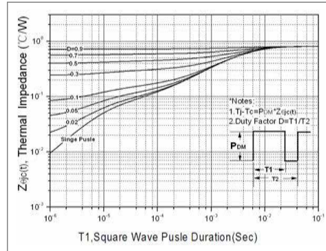
Fig. 12. Transient thermal response curve (TO-251N)
